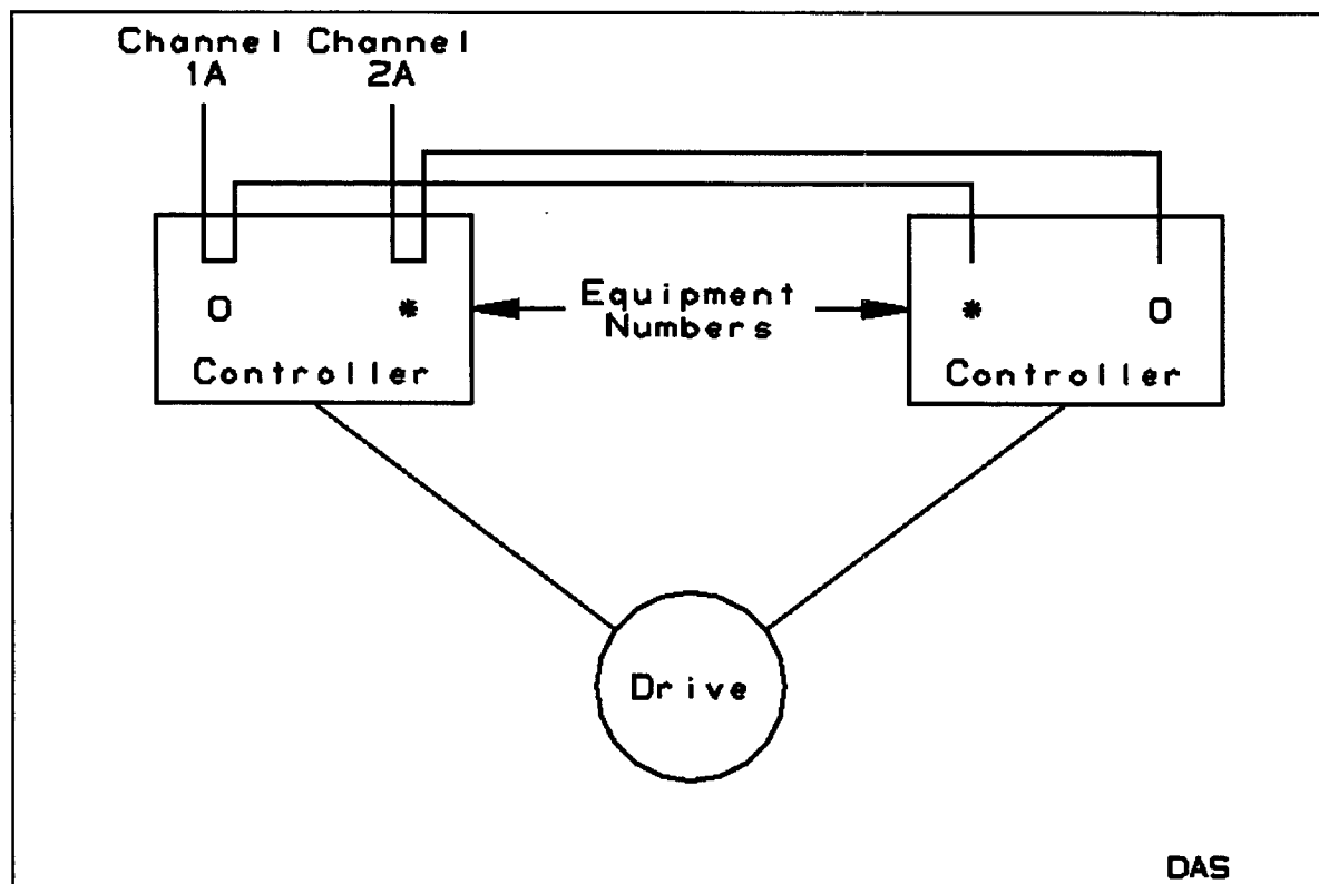
Figure 3-6. Dual-Channel Access to 5830 Drives
