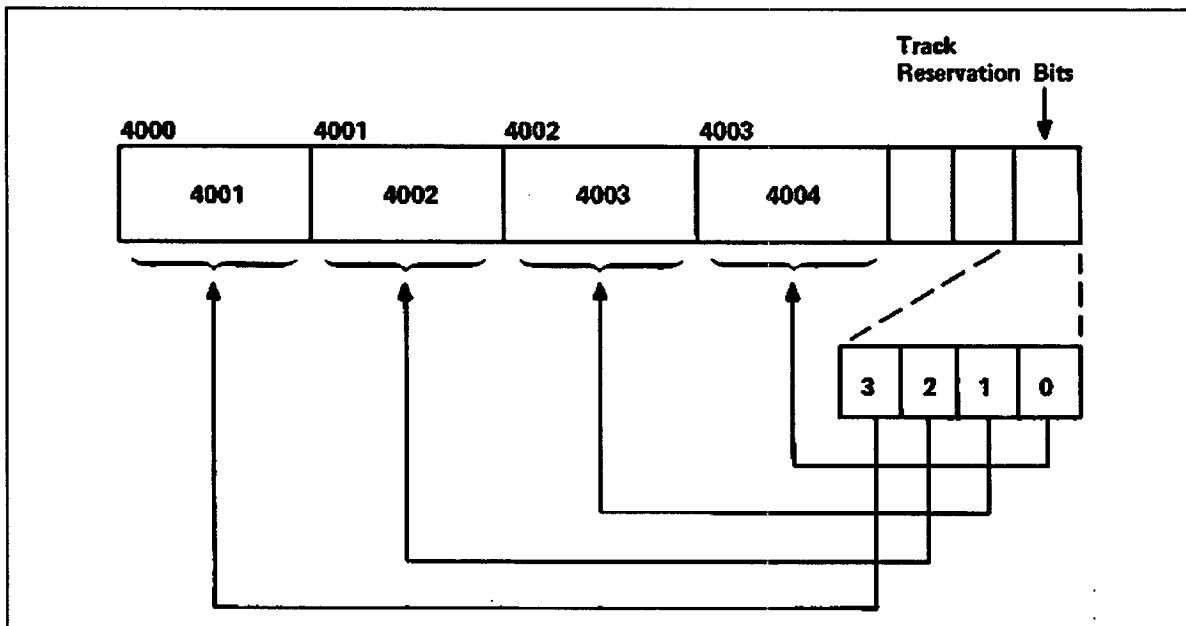
Figure 17-3. Bit Settings for Track Link Bytes
