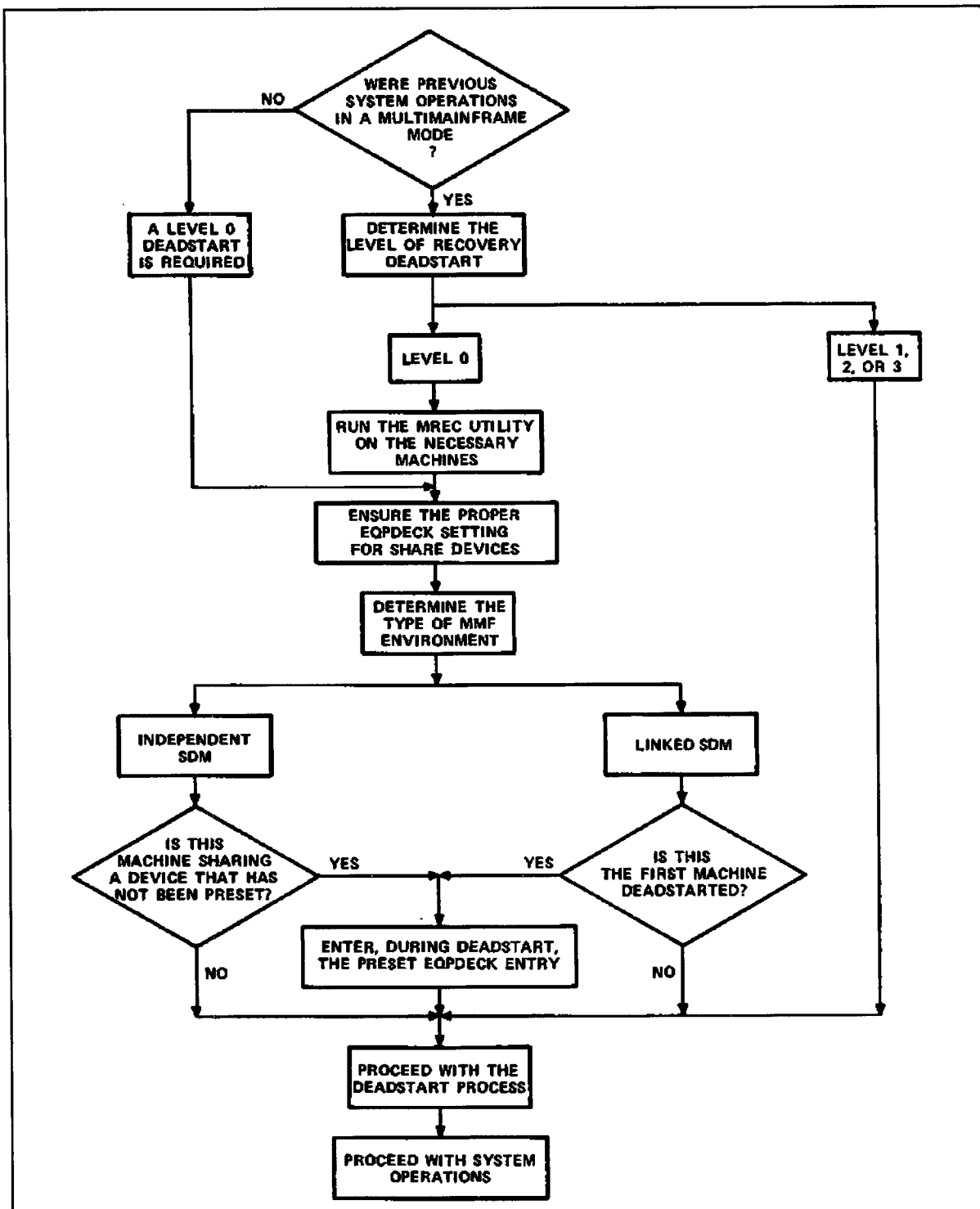
Figure 13-1. Deadstarting a Machine in a Multiframe Complex
