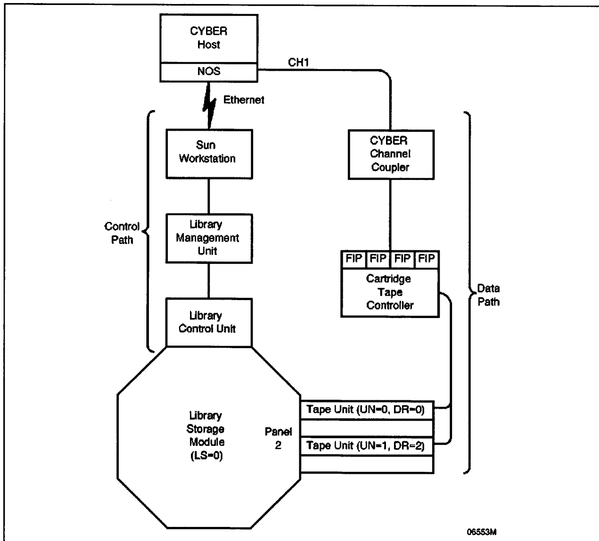
Figure 22-4. ACS Minimum Configuration
